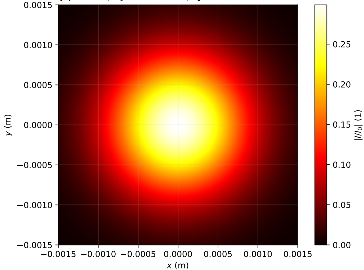
Intensity profile I(x, y, z = 3.264m)/I_0 , P_{in}=0.1P_{cr} , artificial time
